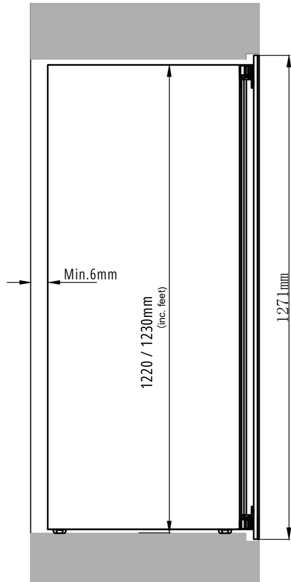
Side View
